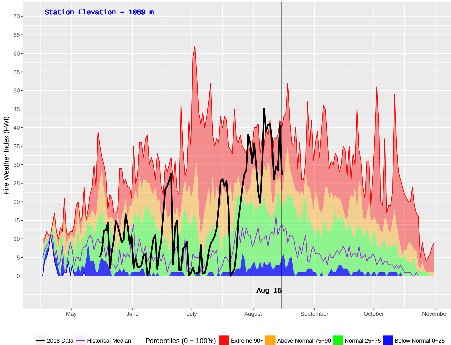
EAST OOTSA (170) : Historical (1986–2016) and Current (2018) Daily Fire Weather Index (FWI)
