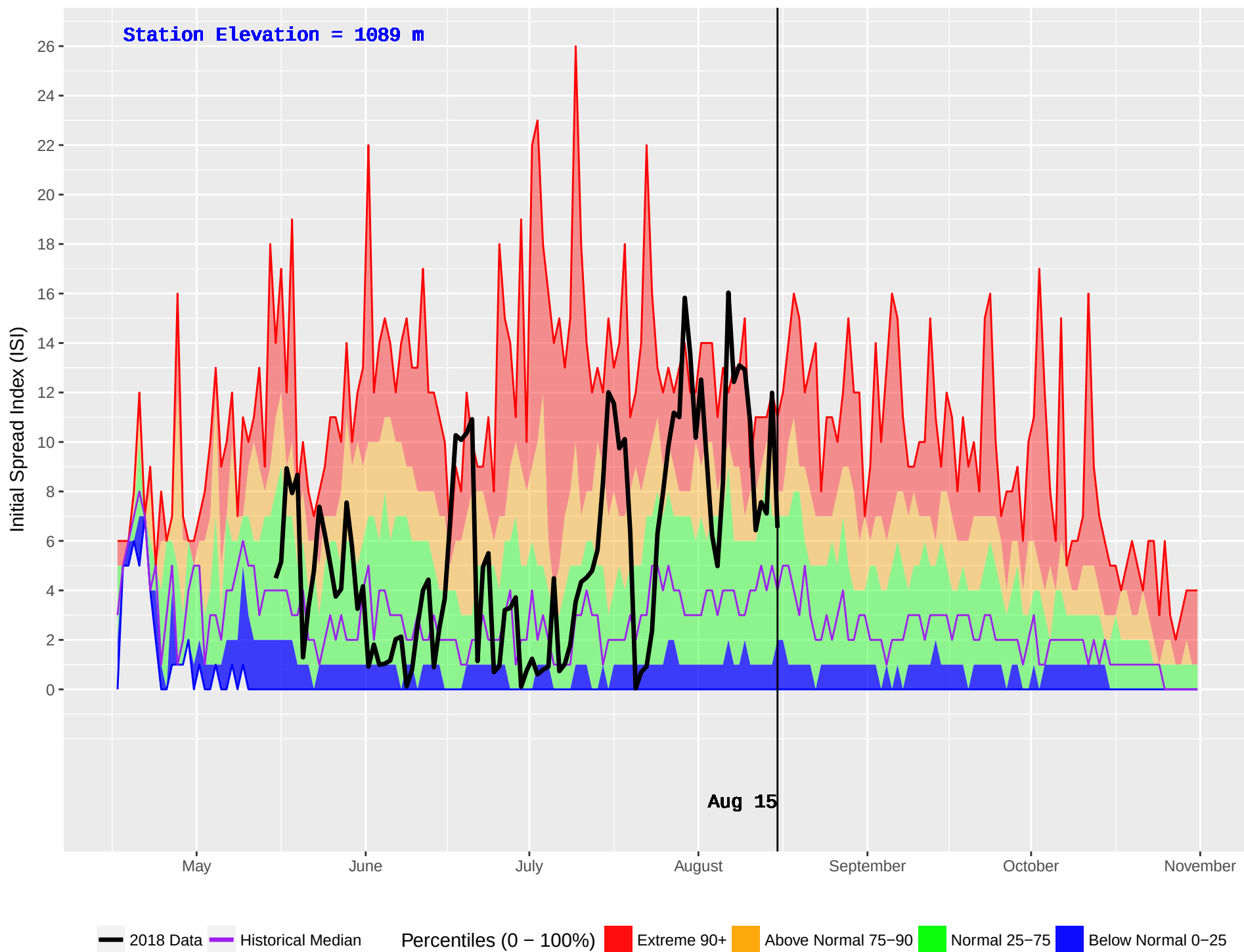
EAST OOTSA (170) : Historical (1986–2016) and Current (2018) Daily Initial Spread Index (ISI)
